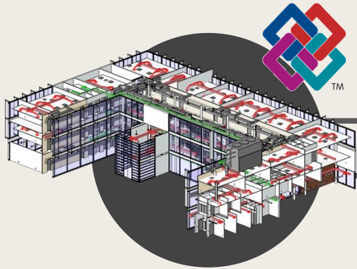
IFC 3D Digital Model: Most 3D Modelling Software
